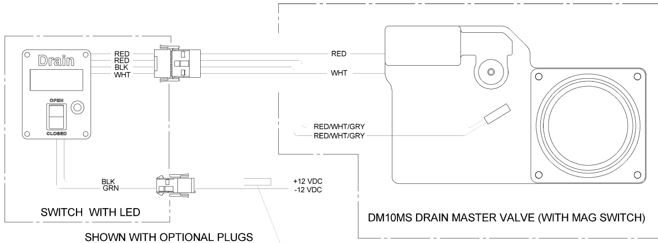
GLASS TYPE FUSE MDL-5 OR AUTOMOTIVE BLADE TYPE 5.0 AMP Wiring Diagram
